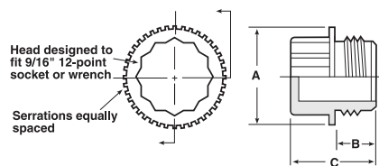
Straight Thread Caplugs Nos. P-18B thru P-68B
