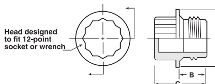
Straight Thread Caplugs No. P-48C
