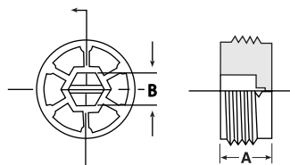
Straight Thread Caplugs No. P-68VH
