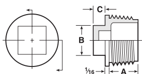
Tapered Thread Caplugs Nos. P-68H and P-88H
