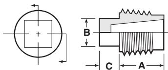
Tapered Thread Caplugs Nos. P-18 thru P-128
